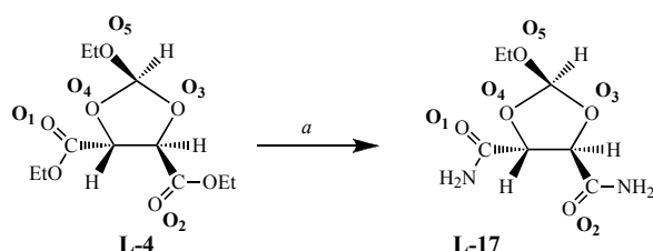
Scheme 5 Synthesis of L-2-ethoxy-1,3-dioxolane-4,5-carboxamide L-17 . a) \text{CH}_3\text{OH} , \text{NH}_3\text{aq} , rt, overnight, 100%.
