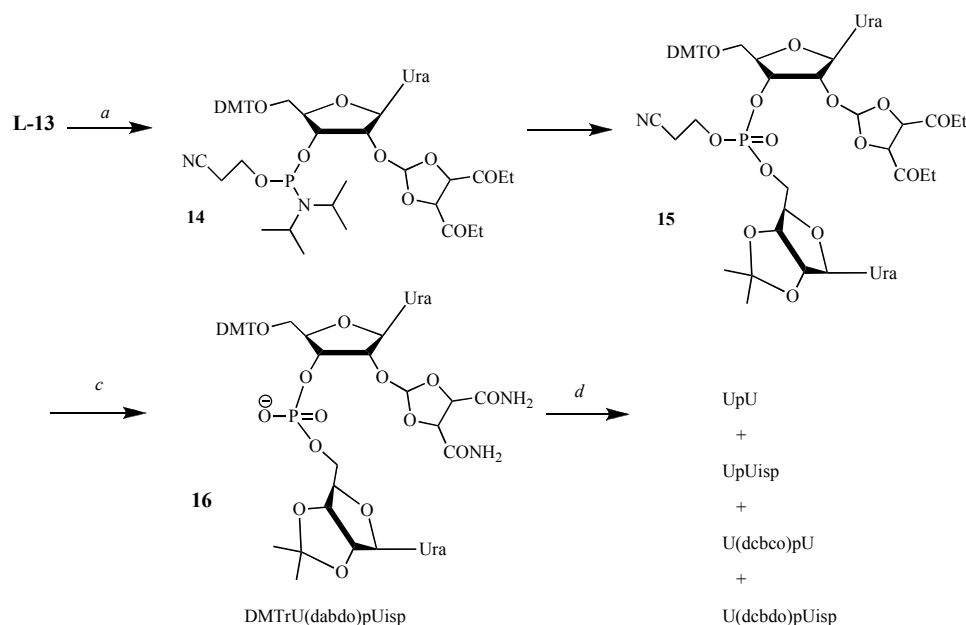
Scheme 4 Synthesis of UpU by the 1 H -tetrazole-mediated reaction of 2',3'- O -isopropylideneuridine with 1,3-dioxolane-4,5-dicarboxylic acid diethyl ester. a) \text{CH}_2\text{Cl}_2 , rt, (i\text{Pr})_2\text{NEt} , chloro(2-cyanoethoxy)diisopropylaminophosphine, overnight, 60%; b) i) \text{CHCl}_3 , 2',3'- O -isopropylideneuridine, 1 H -tetrazole; ii) \text{I}_2\text{-H}_2\text{O-Py} ; c) \text{NH}_3\text{aq} ; d) 25% of \text{CD}_3\text{COOD} in \text{D}_2\text{O} .
