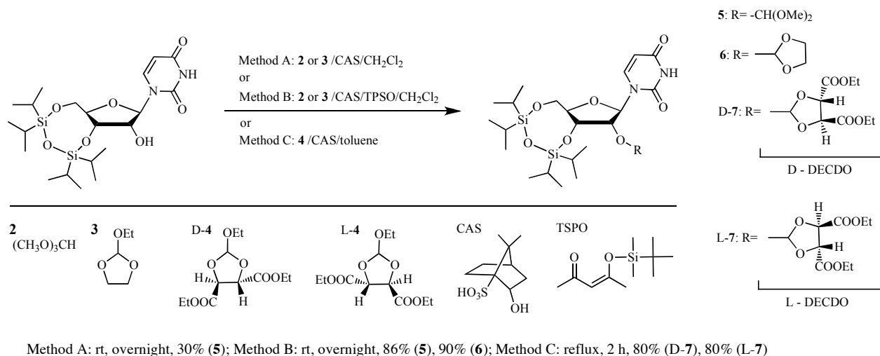
Scheme 2 Synthesis of 2'-O-dialkoxyethyluridine derivatives.
