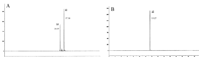
Figure 1 Chart A: RP HPLC trace of the mixture 15 and 16 synthesized using the monomers 14 (solvent system I), Chart B: RP HPLC profile of the mixture obtained by treatment of 16 with 25% \text{CD}_3\text{COOD} in \text{D}_2\text{O} (Solvent system II).
