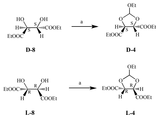
Scheme 1 Synthesis of 2-Ethoxy-1,3-dioxolane-4,5-dicarboxylic acid diethyl ester and 2-Ethoxy-1,3-dioxolane-4,5-dicarboxylic acid diamide. a) Toluene, CAS, 95 °C, 95%.
