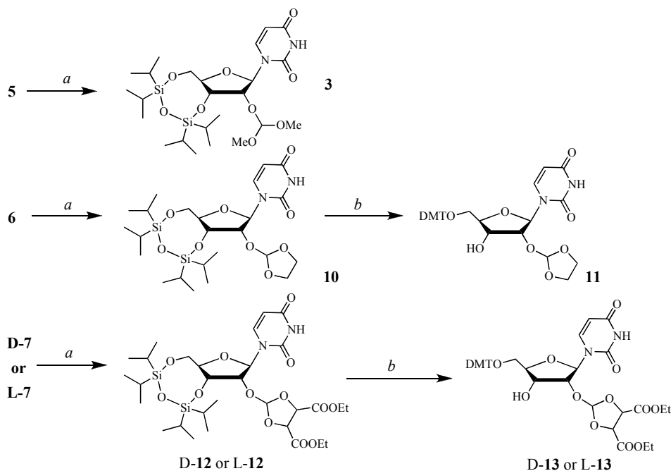
Scheme 3 a) THF, TBAF, RT, 30 min, 95% ( 10 ), 95% (D- 12 ), 98% (L- 12 ); b) DMT-Cl, pyridine, rt, 4h, 64% ( 11 ), 2 h, 94% (D- 13 ), 2h, 96% (L- 13 ).
